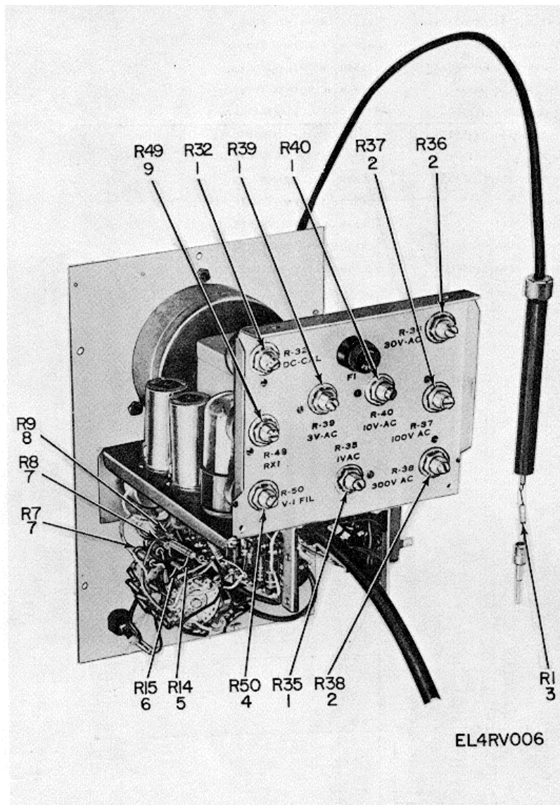
Figure 6. ME-26B, C, D/U Multimeters, Chassis, Rear View.
